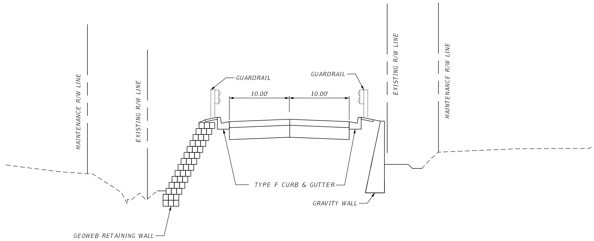
PROPOSED TYPICAL SECTION DELEON ST.
