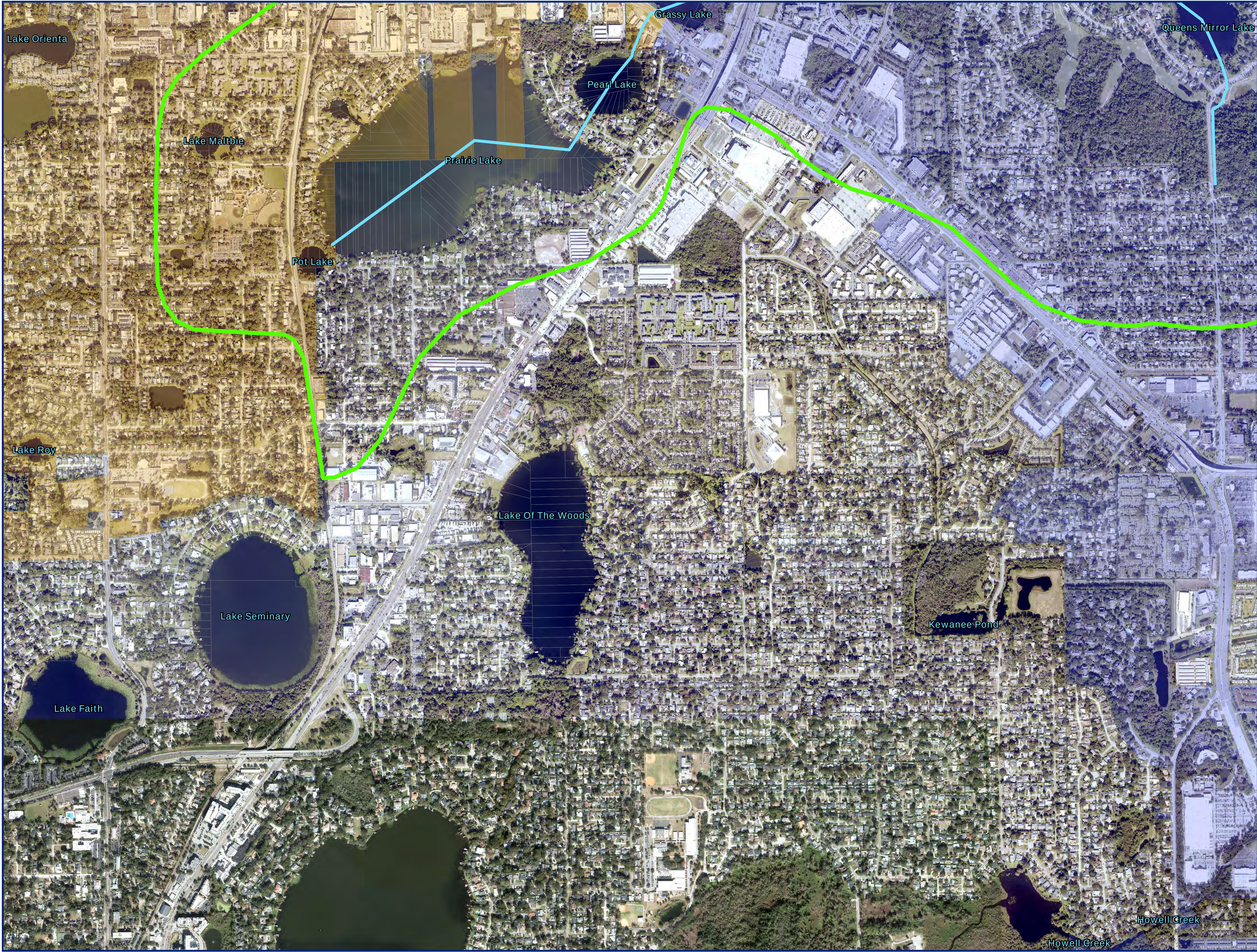
FIGURE E01 GROUP A DRAINAGE BASINS SOLDIERS CREEK, GEE CREEK, AND LITTLE LAKE HOWELL BASIN STUDY
